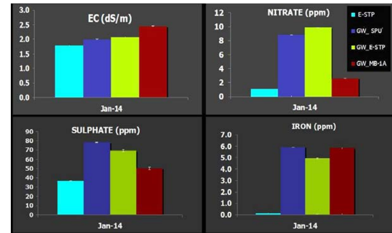
Figure 5: Quality of treated wastewater (e-STP) vs. local groundwater on the Indian Agricultural Research Institute farm
