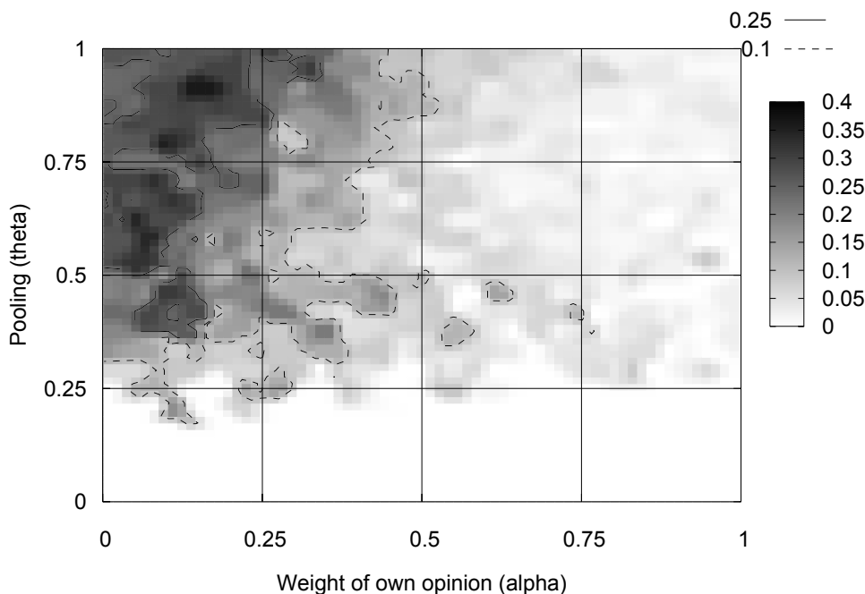
Figure 4: Cliquishness of the emerging network in the (\alpha, \theta) -space.
