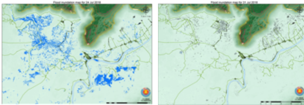
Figure 10.9 Flood Inundation Area in Sanamxay District on 24 July (left) and 31 July 2018 (right)
