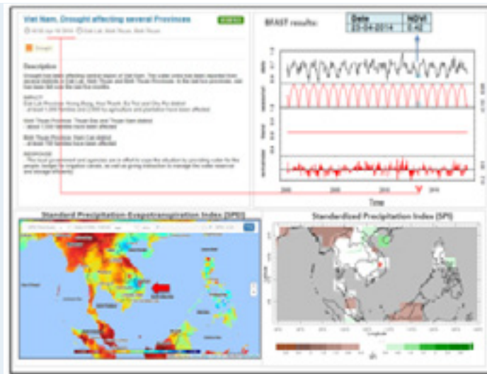
Figure 6.4 SPEI and SPI for the drought in Dak Lak, Viet Nam
