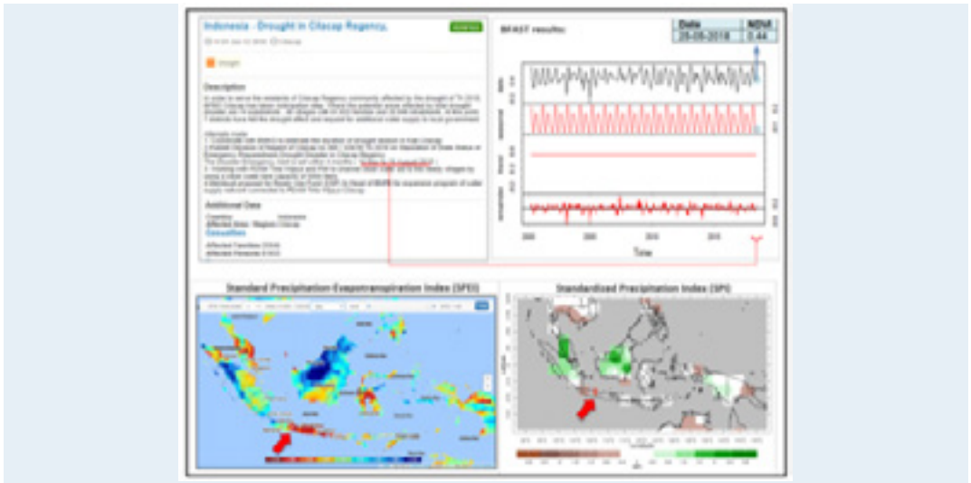
Figure 6.2 SPEI and SPI for the drought in Cilacap, Indonesia
