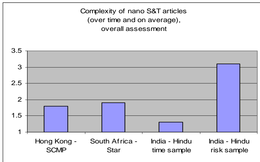
Figure 4.3 Quantifying complexity
